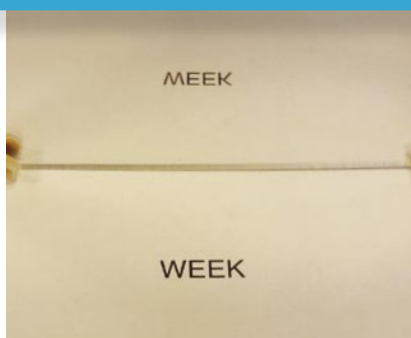
Figure 11 - 'WEEK' viewed through a mirror.
