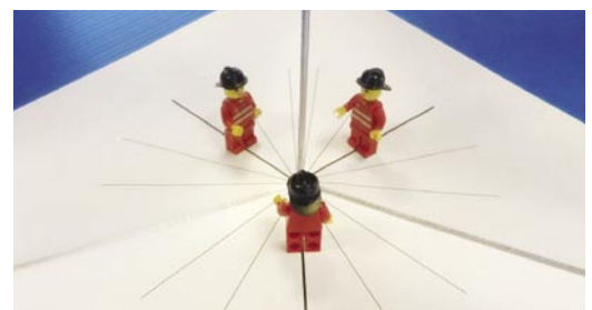
Figure 4 - Mirrors set at an obtuse angle.
