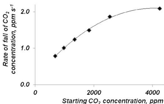
Figure 8 The rate of fall of CO 2 concentration in the chamber as a function of initial CO 2 concentration
