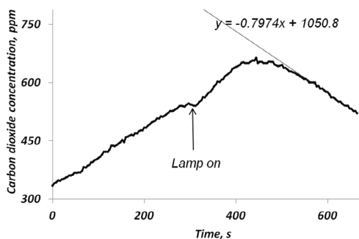
Figure 7 The CO 2 concentration in the chamber as the experiment progressed
