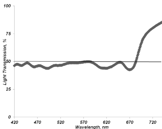
Figure 4 Light transmission of a neutral density 209 filter from Lee Filters. Data are displayed as the percentage of light transmitted as a function of wavelength at 1 nm intervals. The horizontal line represents 'pure' 50% transmission.
